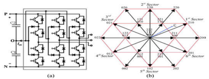
Fig. 8. A typical three-level inverter (a) structure of circuit, and (b) three-level inverter space vector diagram for balanced DC-link capacitors
