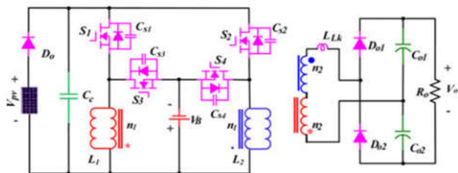
Fig. 3. Three port DC-DC converter
