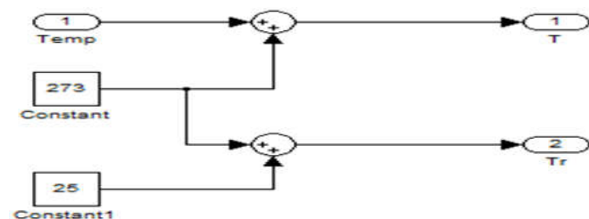
Fig. 7. Simulink model of the temperature conversion from degree Celsius unit to Kelvin unit
