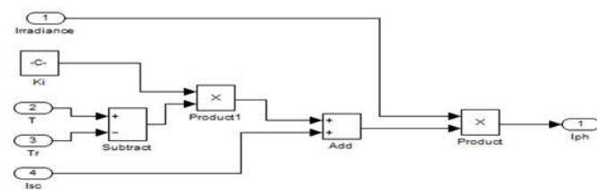
Fig. 6. Simulink model of photocurrent
