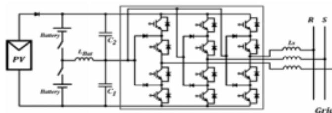
Fig. 2. Circuit Diagram
