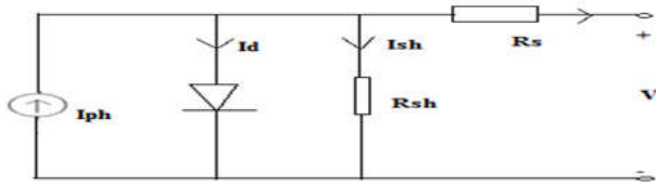
Fig.5 Equivalent circuit of Solar Cell
