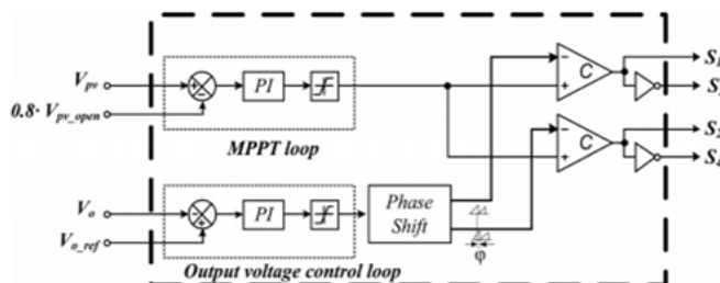
Fig. 4. Diagram of the proposed control scheme
